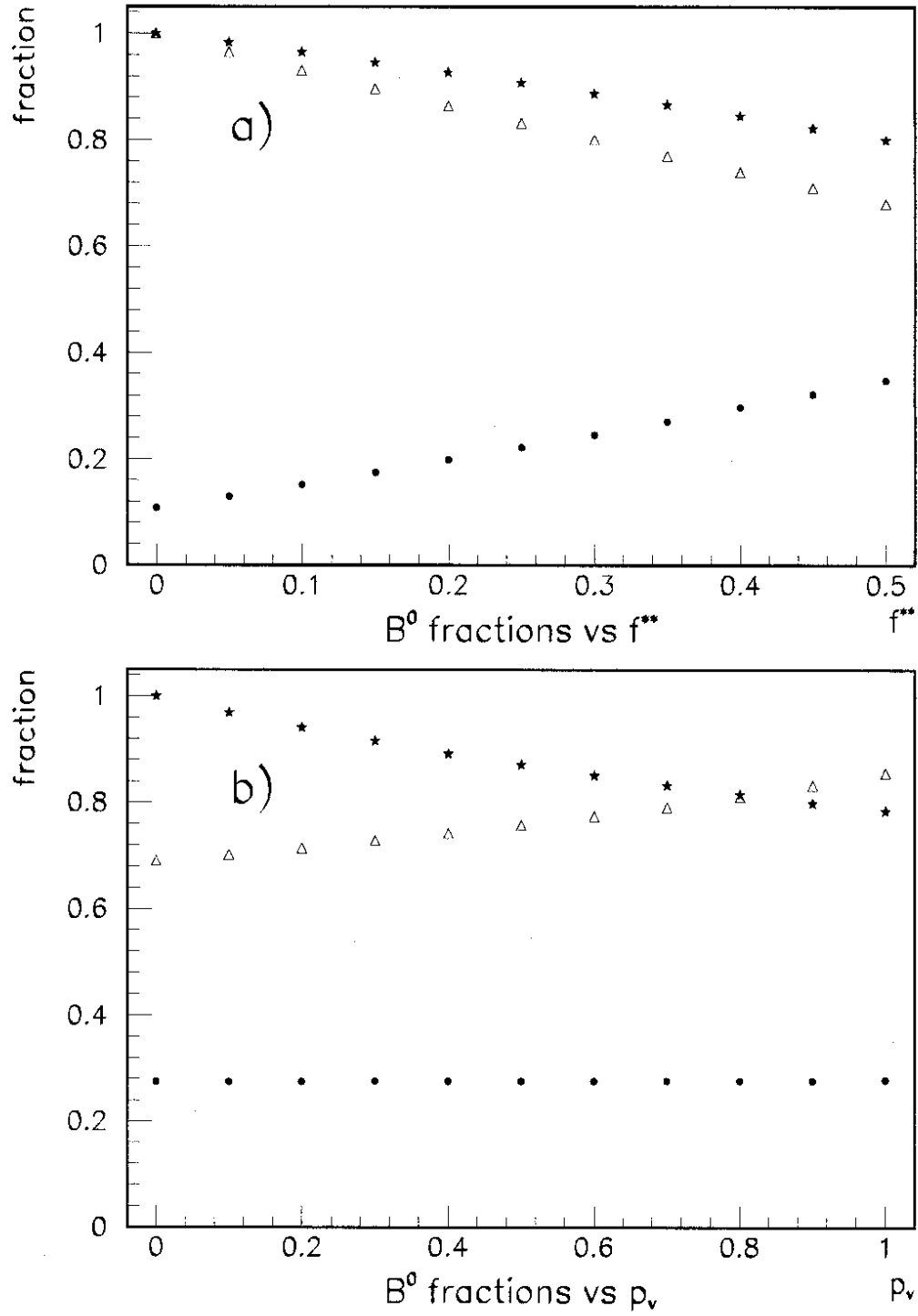
Figure 5: Predicted fraction of B^0 mesons in the samples of \bar{D}^0 \ell^+ events ( \bullet ), D^- \ell^+ events ( \triangle ) and D^{*-} \ell^+ events ( \star ) as a function of (a) f^{**} with p_{\nu} = 0.54 and (b) p_{\nu} with f^{**} = 0.36 .
